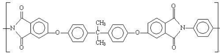
Figure 3. Polyetherimide Structure
