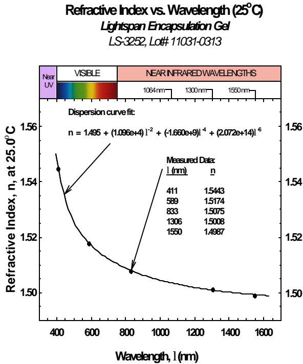
Figure 4, Refractive Index vs. Wavelength
