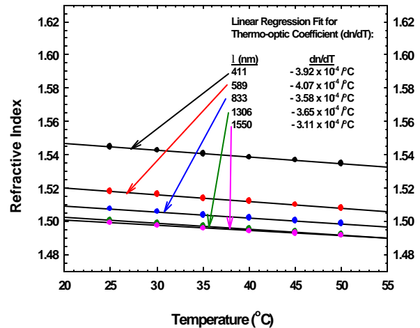
Figure 3, Refractive Index vs. Temperature
