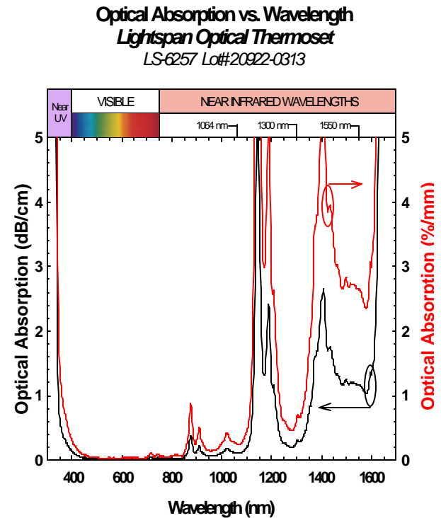
Figure 5, Optical Absorption vs. Wavelength
